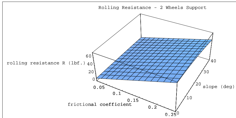
Figure A-6: Rolling resistance as a function of an empirical coefficient of friction f_r and the slope angle \theta (deg) (wheel loading W_w=275 lb).
