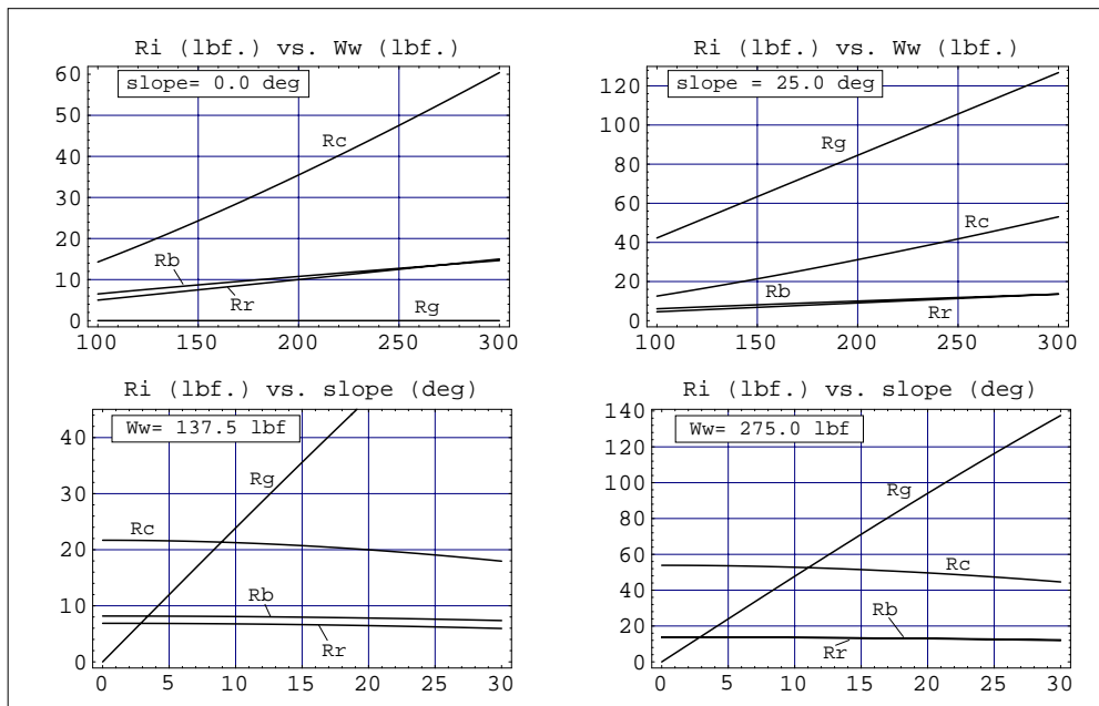
Figure A-10: Compaction R_c (lbf) / Bulldozing R_b (lbf) / Rolling R_r (lbf) / Gravitational R_g (lbf) resistance as a function of wheel loading W_w (lbf) in the upper row ( \theta= 0 deg and \theta= 25 deg) and slope angle \theta (deg) in the lower row ( W_w= 137.5 lbf and W_w= 275 lbf). In all cases: D= 20" , B_w= 15.75' , f_r= 0.05 .
