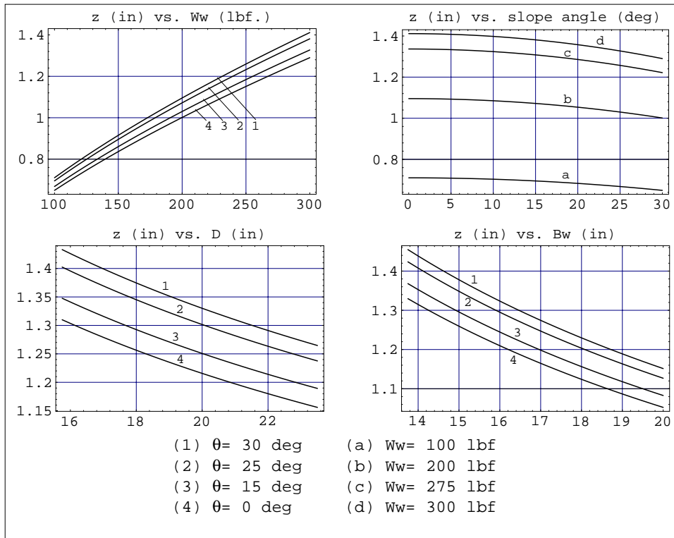
Figure A-2: Wheel sinkage z (in) in dry sand as a function of wheel loading W_w (lbf) and the slope angle \theta (deg) in the upper row (in both cases D=20" , B_w=15.75" ), and wheel diameter D (in) and tire width B_w (in) in the lower row (in both cases wheel load W_w=275 lbf).
