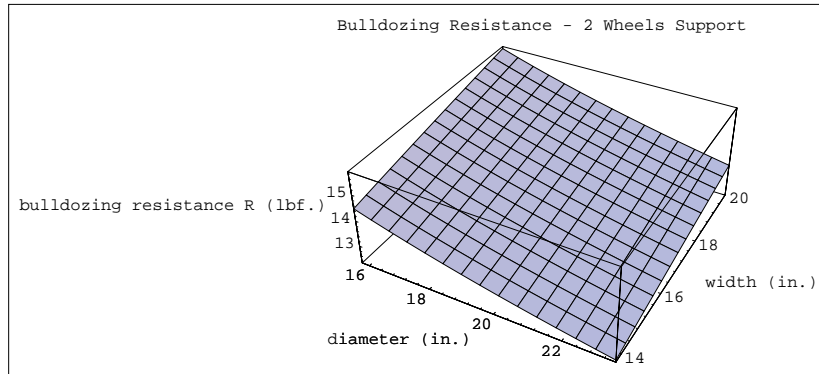
Figure A-5: Bulldozing resistance R_b (lb) of a rigid wheel as a function of wheel diameter D (in) and tire width B_w (in) (wheel loading W_w=275 lb).
